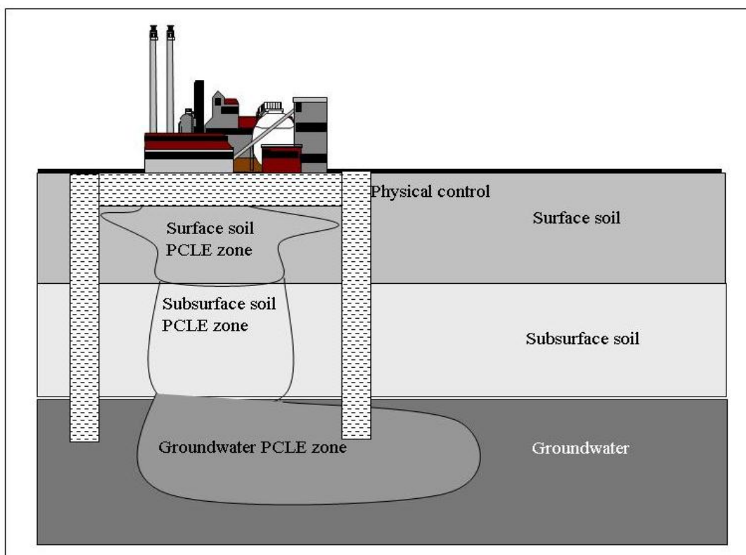
Figure 12. Remedy Standard B surface and subsurface soil response objectives under §350.33(e)(2) using removal and/or decontamination with controls or controls only. This is an example of the physical control measures that may be used. The vertically oriented physical controls addressing the soil PCLE zones may not be routinely warranted.
