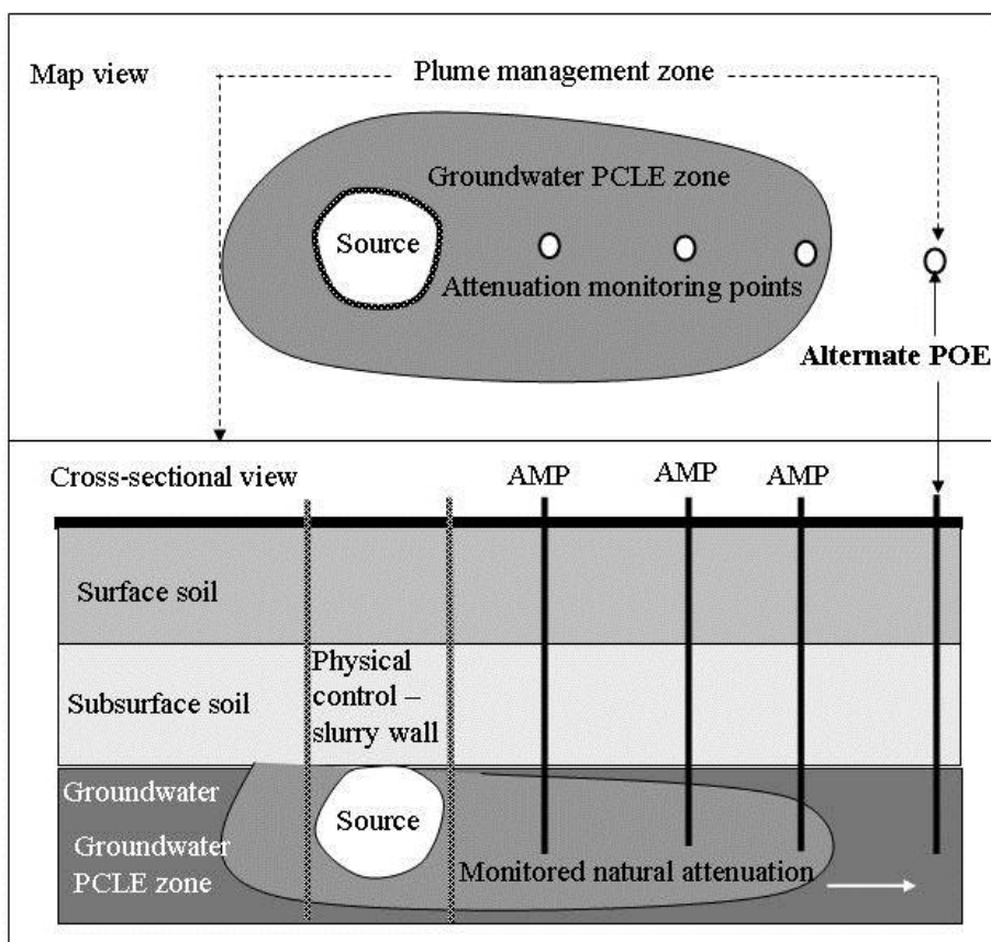
Figure 9. Example of Remedy Standard B plume management zone based on decontamination (monitored natural attenuation) and control (slurry wall). AMP is attenuation monitoring point.
