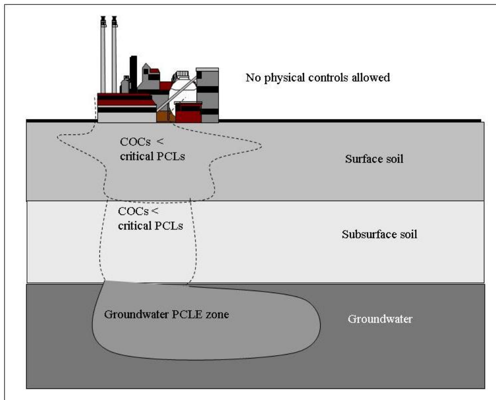
Figure 11. Remedy Standard B surface and subsurface soil response objectives under §350.33(e)(1) using removal and/or decontamination but not control measures. All surface and subsurface soil PCLE zones have been removed.
