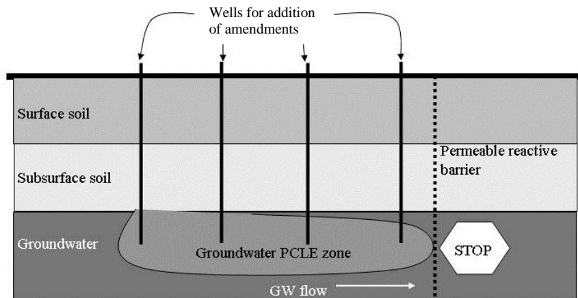
Figure 4. Example of Remedy Standard B groundwater response action based on decontamination (amendments, MNA and/or permeable reactive barrier)
