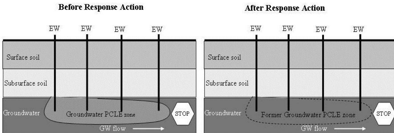
Figure 3. Example of Remedy Standard B groundwater response action based on removal (Groundwater Extraction Wells (EW))
